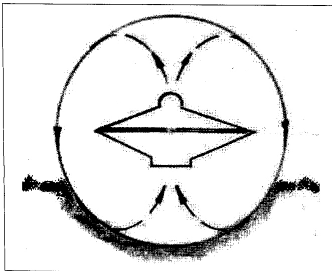
Figure 2 Notice that in this position the force upon the water is pushing downward.
