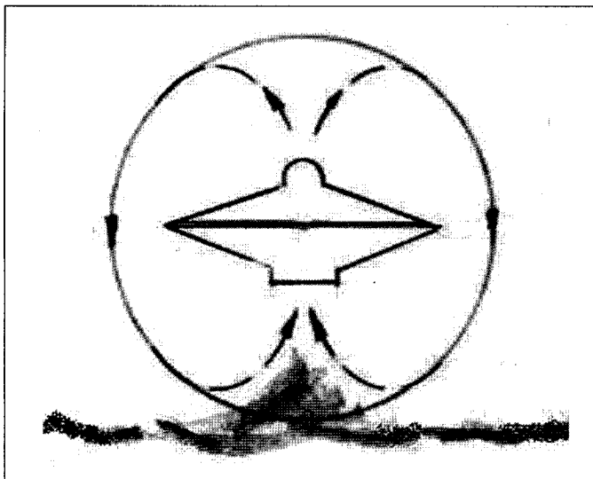
Figure 3 Notice here the water, assuming the shape of the upward flow of the field apparently entering the UFO.
