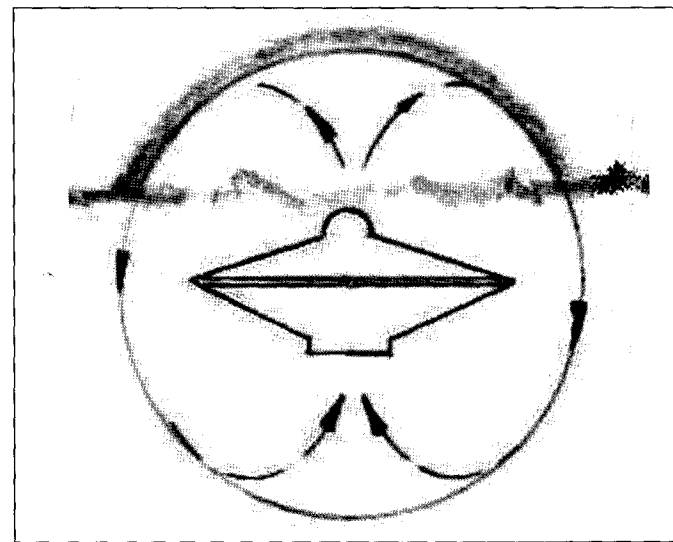
Figure 1 (Underwater) Notice how if this idea is correct, the force is pushing upwards, causing a bulge.
