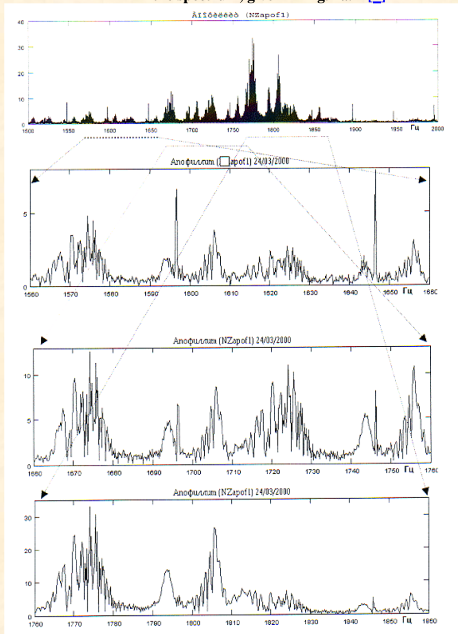
Fig. 2 the PLR-spectrum of a mineral (apofillit). Arrows (pointers) specify area of display of the spectrum, given in Fig. 2a. [2]
