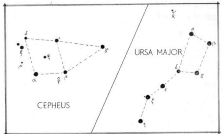
Fig. 2.—The positions of the two Long-Period-Variables, R Ursae Majoris and T Cephei.
