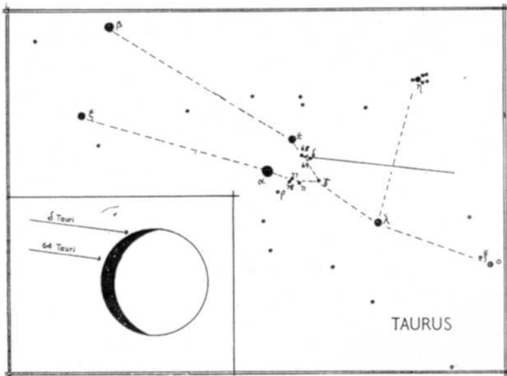
Fig. 1.—The occultation of the stars \delta and 64 Tauri on December 23. The arrow represents the path of the moon as seen from the centre of the earth during the day, and inset shows how the stars will disappear behind the dark edge of the moon as seen from London.
