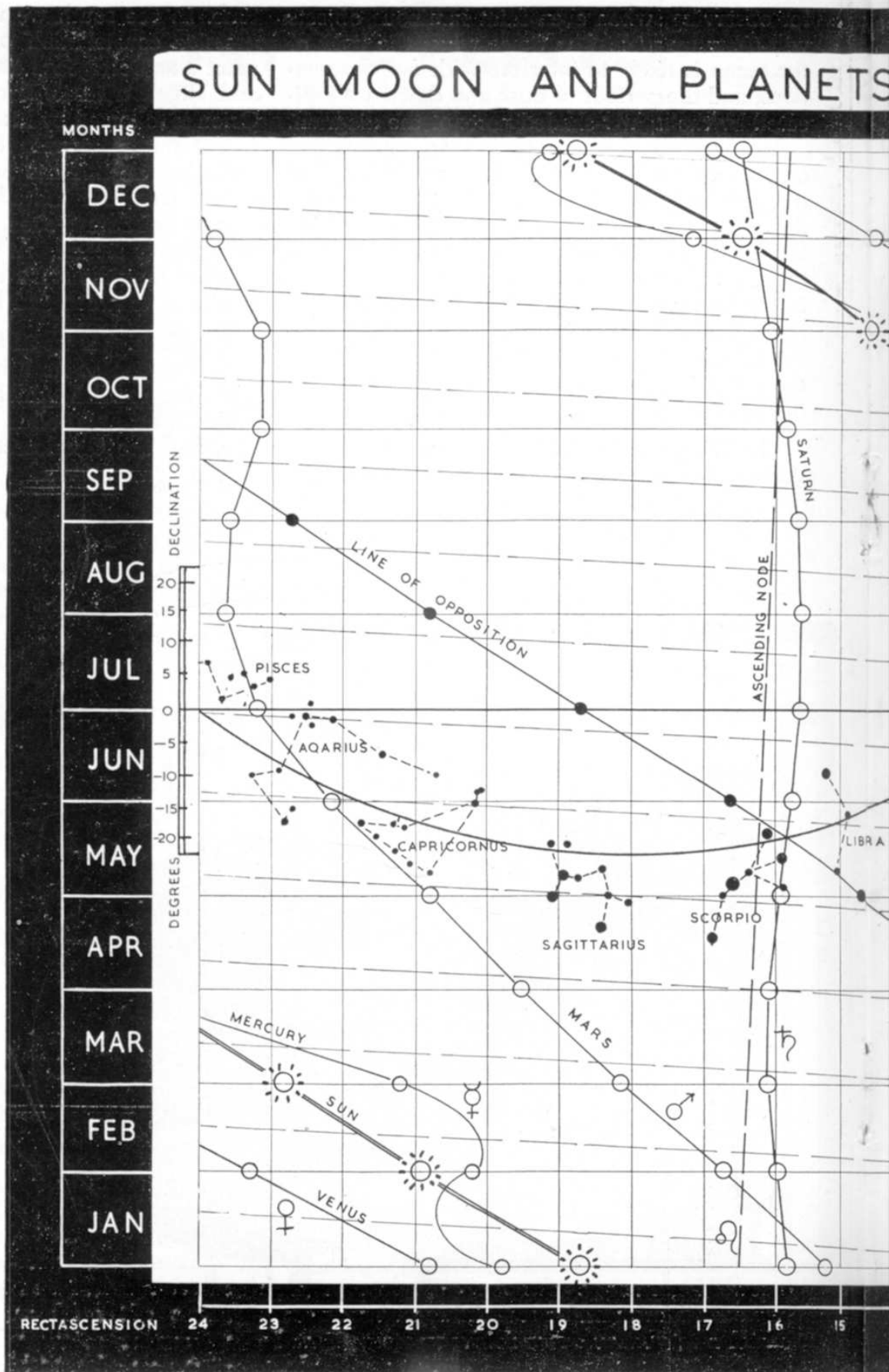
Fig. 3. Astronomical
