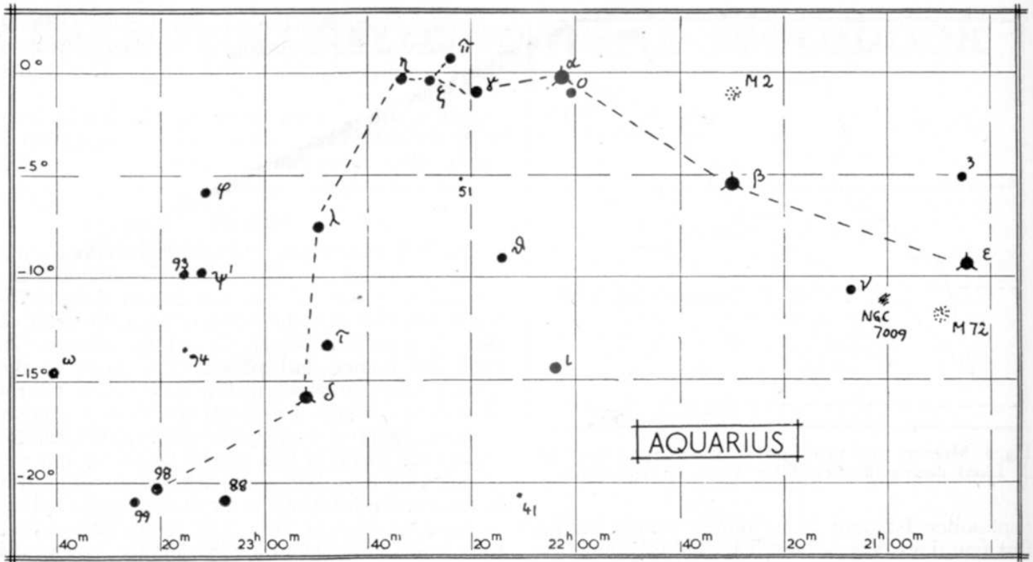
Fig. 3. The constellation Aquarius (The Water Carrier).
