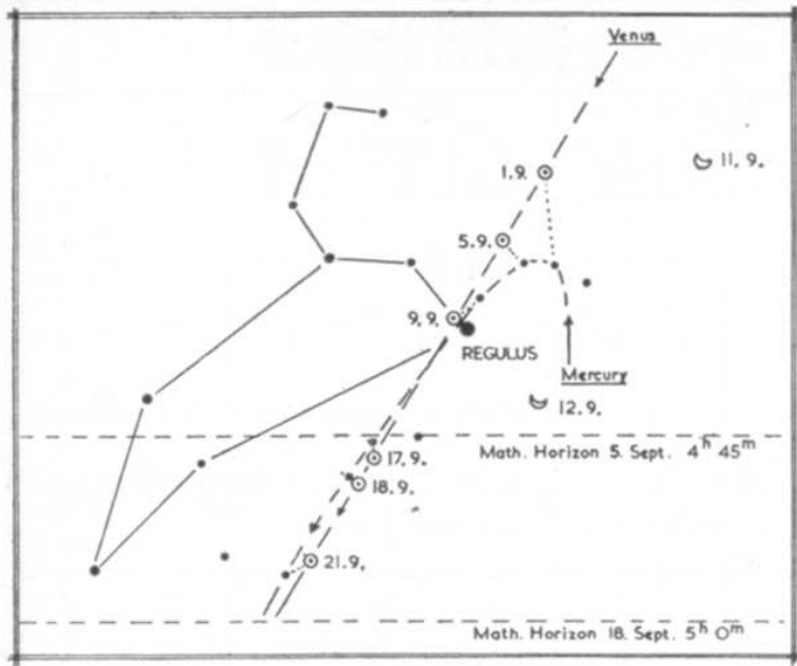
Fig. 1. Mercury and Venus in the constellation Leo (The Lion) during the first three weeks of September.
