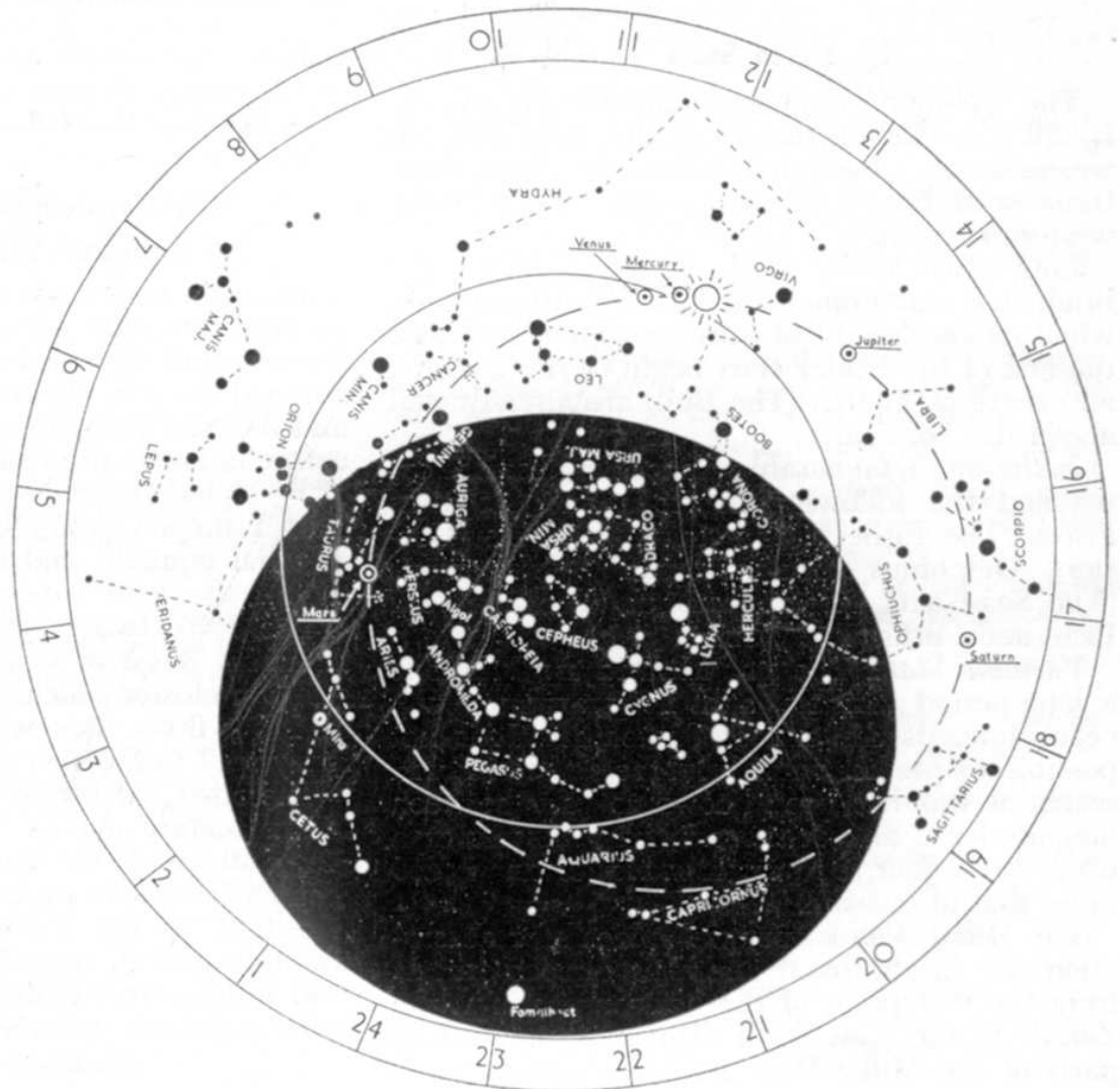
Fig. 2. The night sky on October 1, 1958, at 22.00 hrs. G.M.T.
