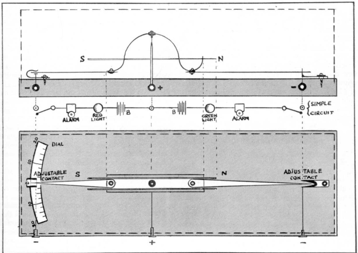
Plan and Side Elevations of the Ufoscope show clearly how the components listed in the text fit into place.
